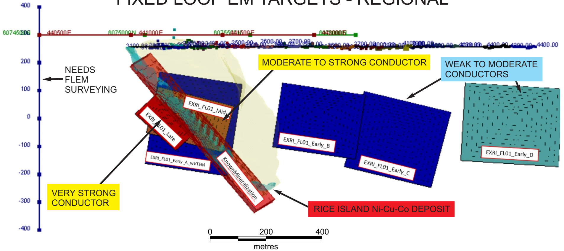
LONGITUDINAL SECTION LOOKING NORTHWEST
